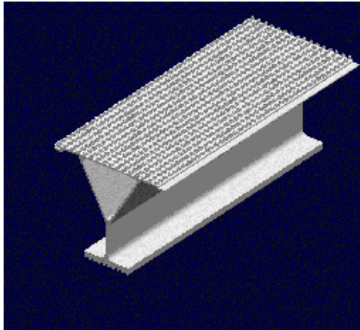
Helideck designed for maximum friction and reduced need for utilization of landing net.
